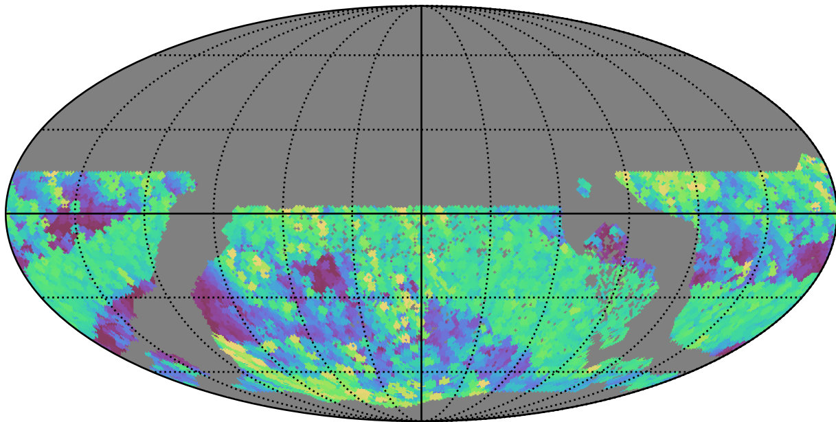
extra_ss_neo3_v3.4_10yrs WFD r band: Max airmass
