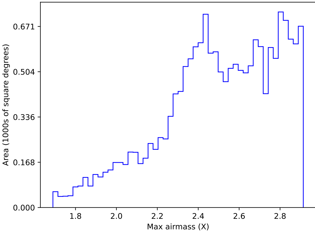
extra_ss_neo3_v3.4_10yrs WFD i band: Max airmass
