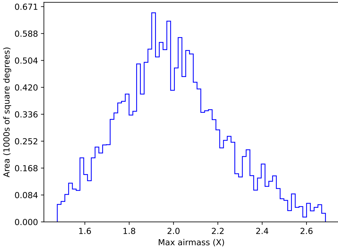
extra_ss_neo3_v3.4_10yrs WFD g band: Max airmass
