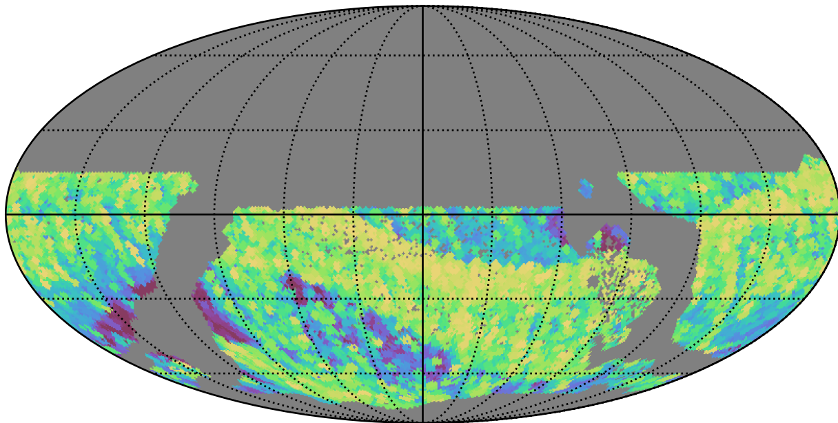
extra_ss_neo3_v3.4_10yrs WFD all bands: Max airmass
