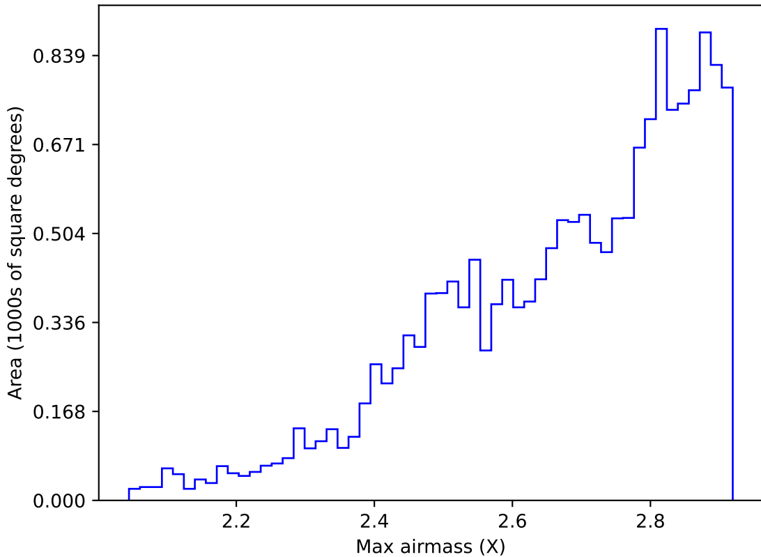
extra_ss_neo3_v3.4_10yrs WFD all bands: Max airmass
