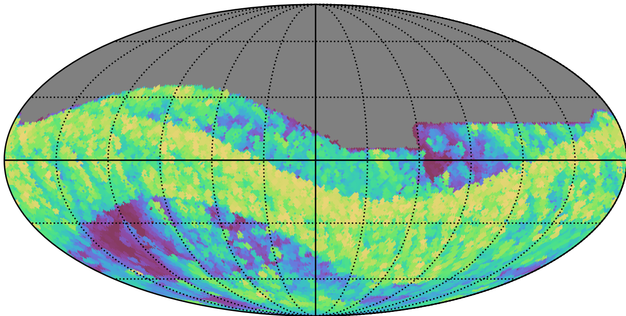
extra_ss_neo3_v3.4_10yrs All sky z band: Max airmass
