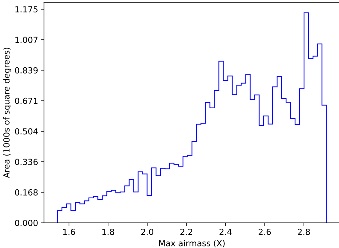
extra_ss_neo3_v3.4_10yrs All sky z band: Max airmass
