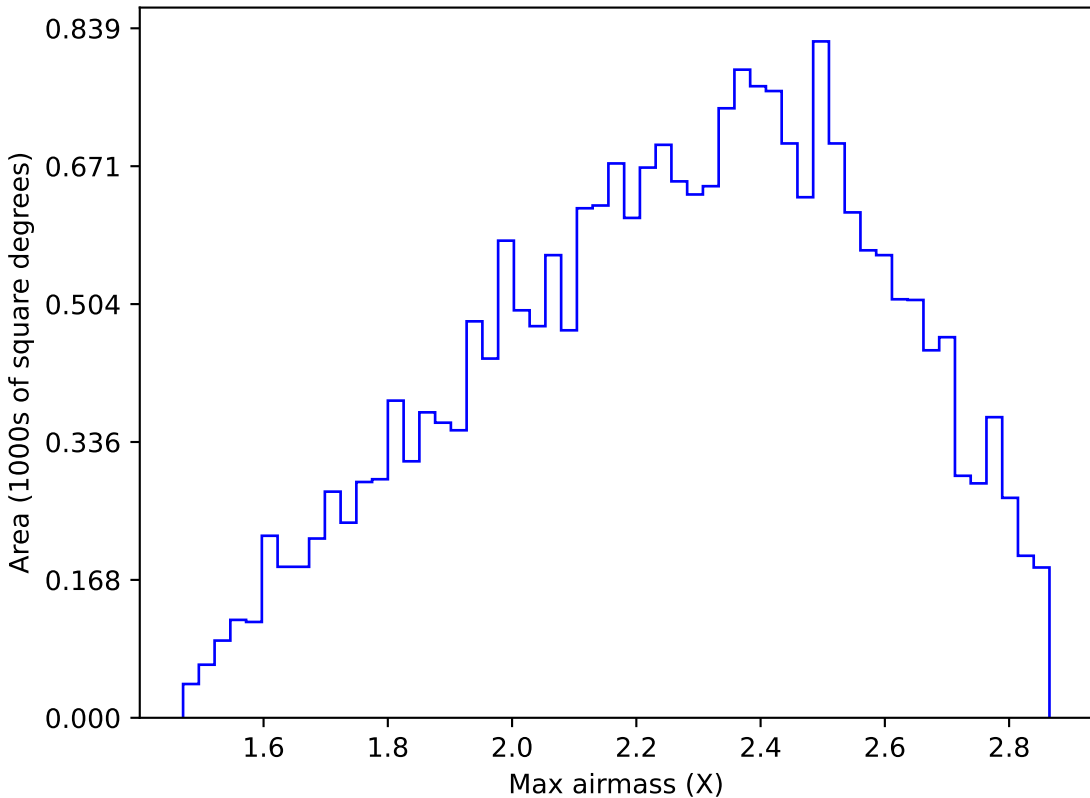
extra_ss_neo3_v3.4_10yrs All sky y band: Max airmass
