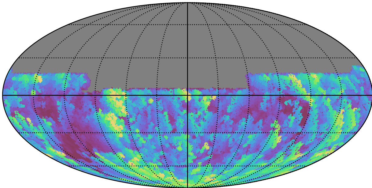
extra_ss_neo3_v3.4_10yrs All sky u band: Max airmass
