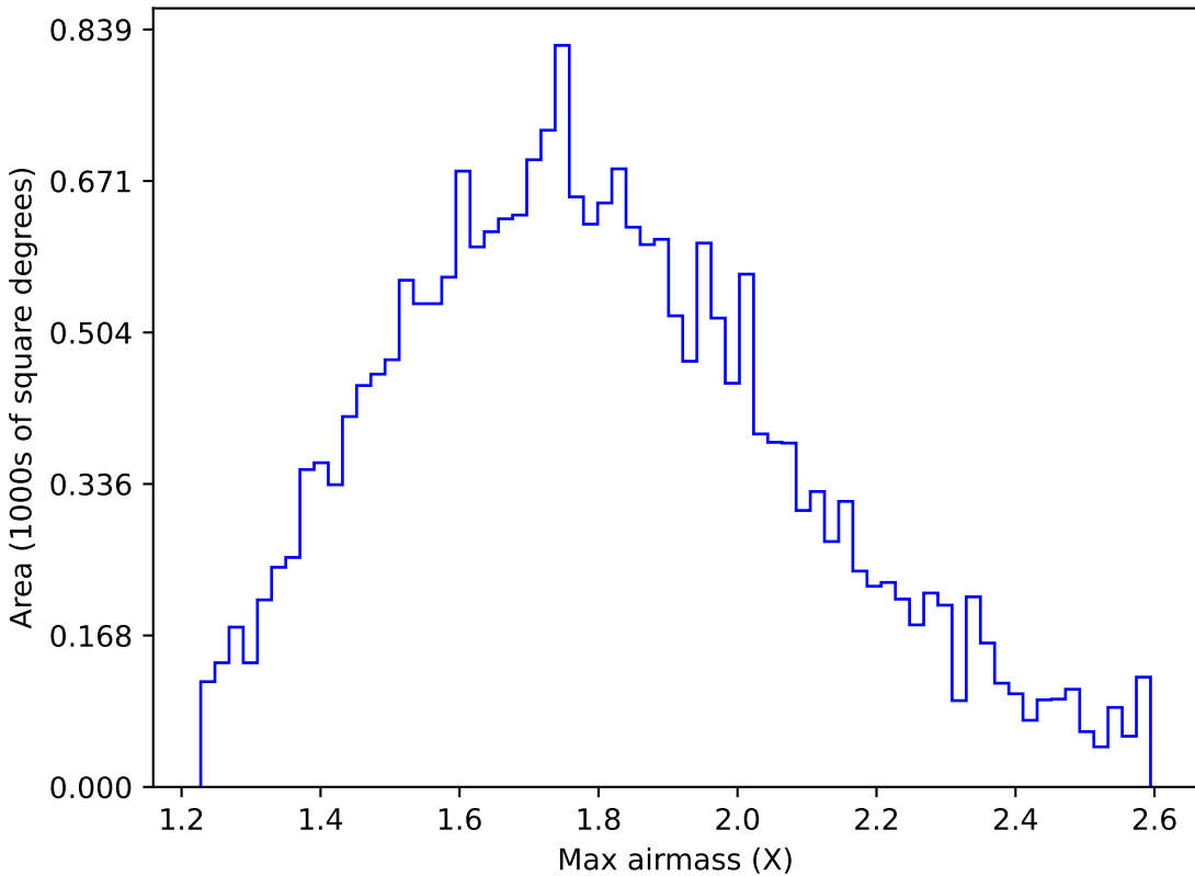
extra_ss_neo3_v3.4_10yrs All sky u band: Max airmass
