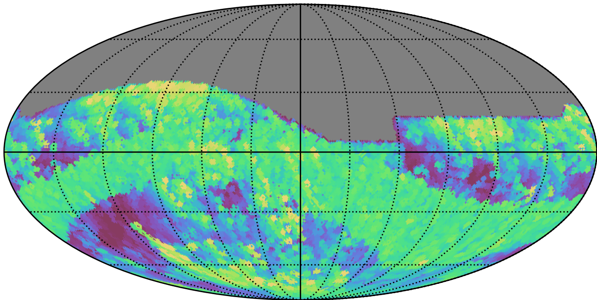
extra_ss_neo3_v3.4_10yrs All sky r band: Max airmass
