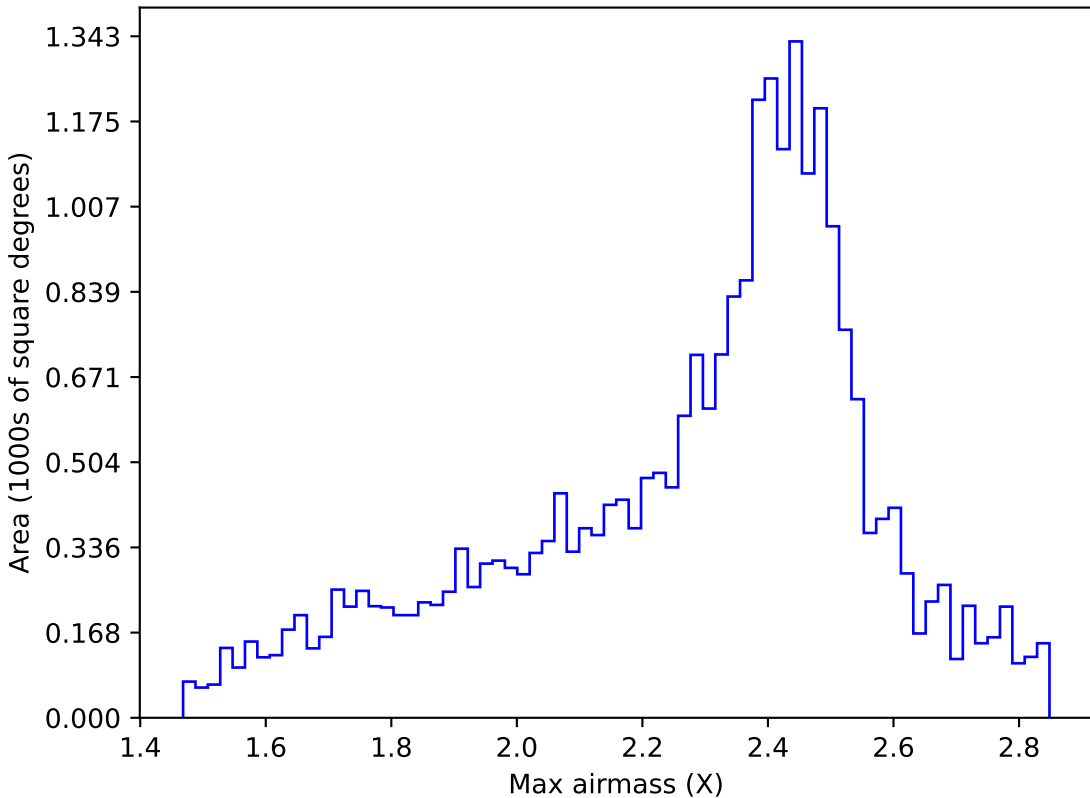
extra_ss_neo3_v3.4_10yrs All sky r band: Max airmass
