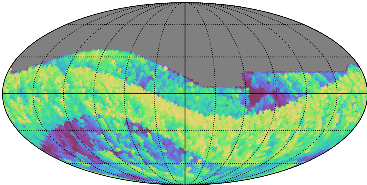
extra_ss_neo3_v3.4_10yrs All sky i band: Max airmass
