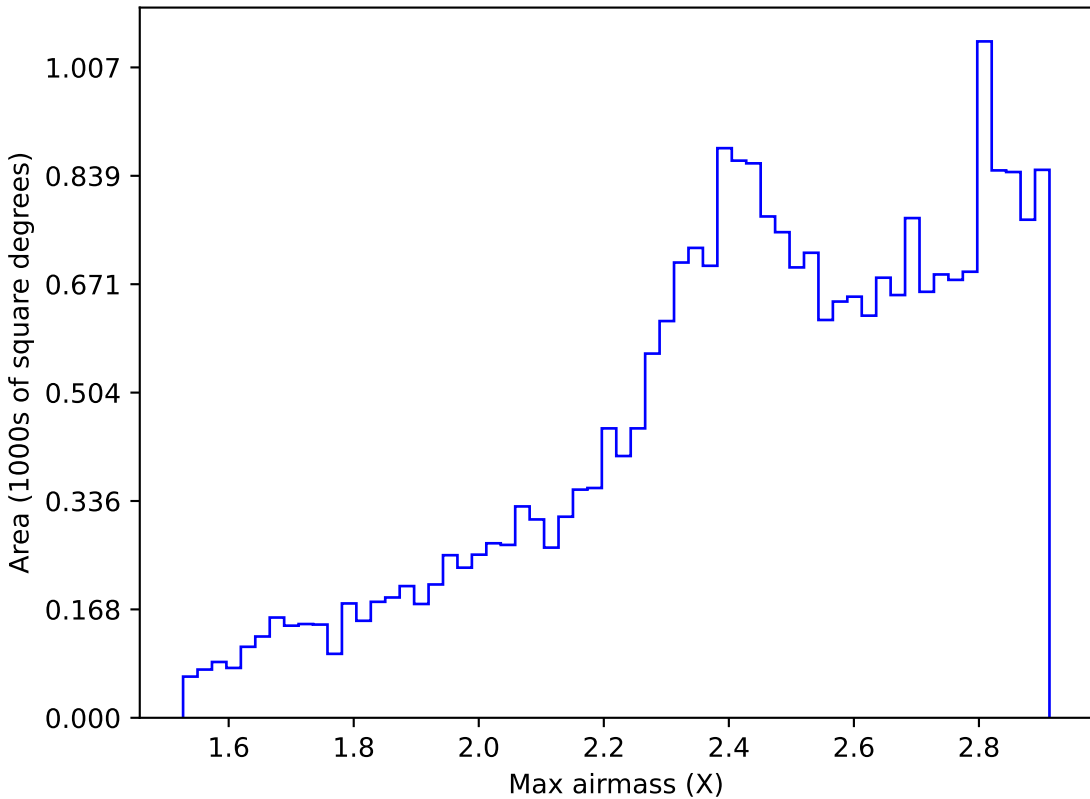
extra_ss_neo3_v3.4_10yrs All sky i band: Max airmass
