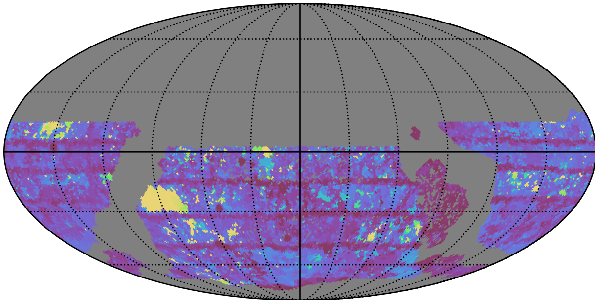
extra_ss_neo3_v3.4_10yrs WFD z band: Max Inter-Night Gap
