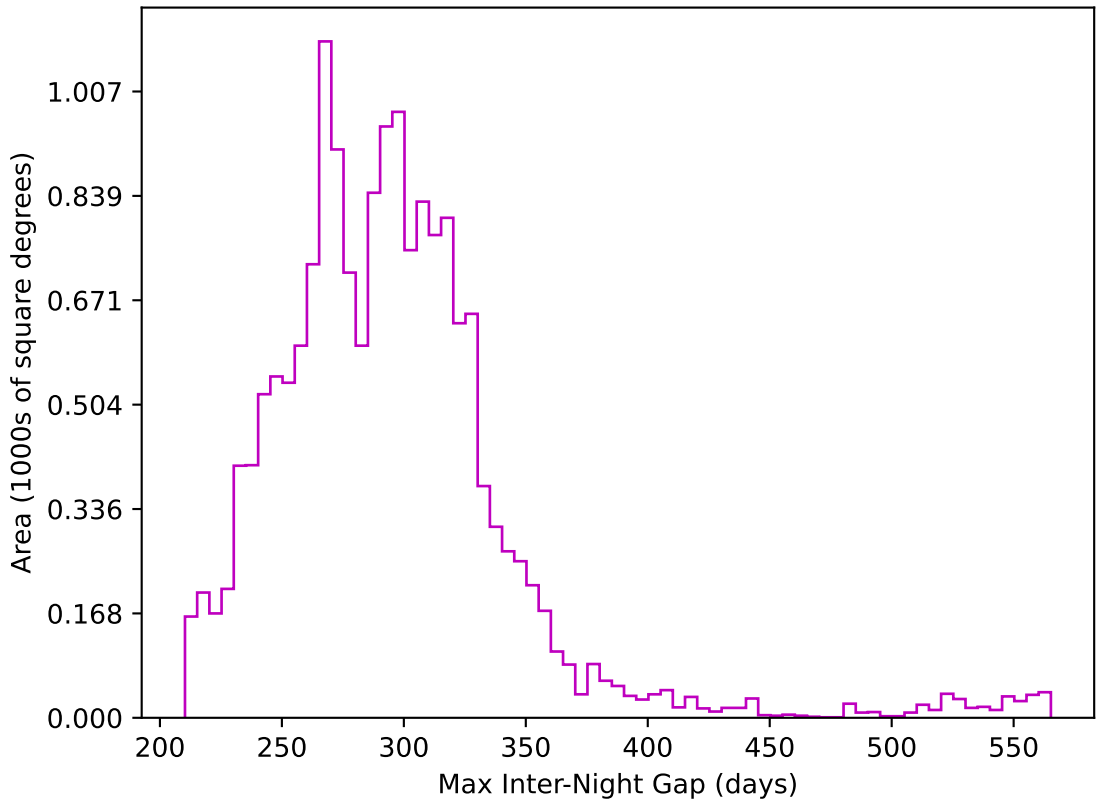
extra_ss_neo3_v3.4_10yrs WFD z band: Max Inter-Night Gap
