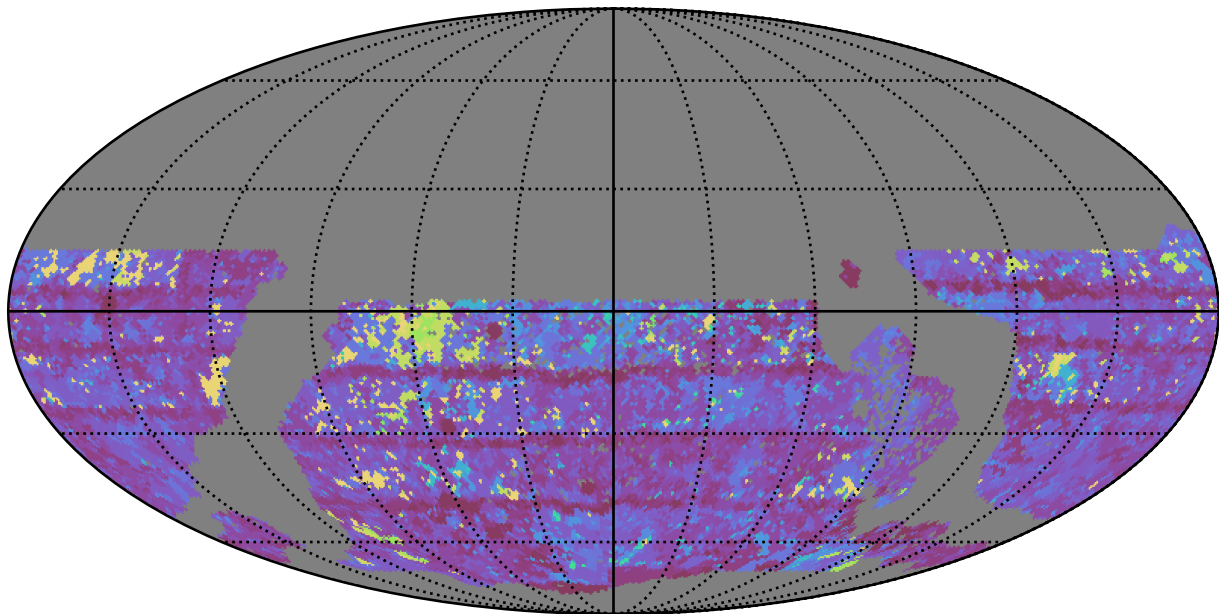
extra_ss_neo3_v3.4_10yrs WFD y band: Max Inter-Night Gap
