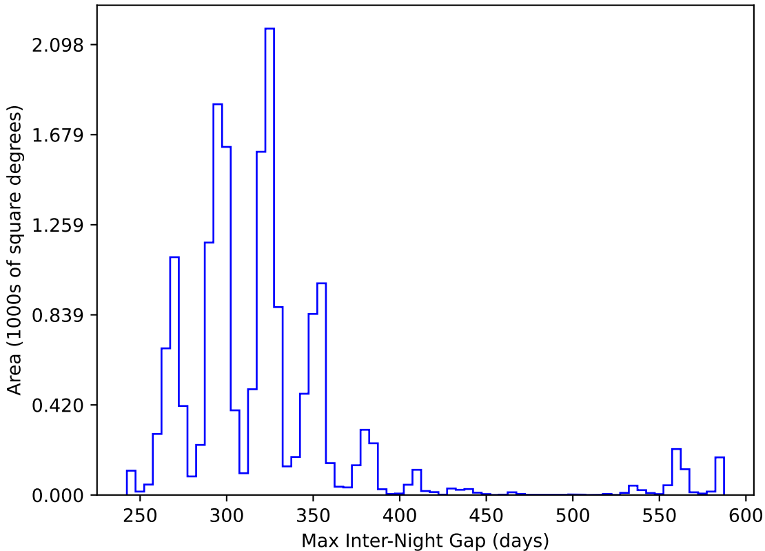
extra_ss_neo3_v3.4_10yrs WFD y band: Max Inter-Night Gap
