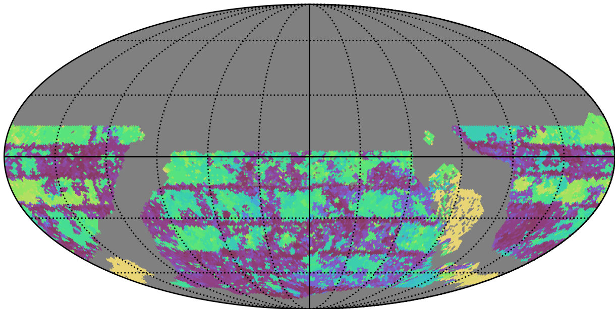
extra_ss_neo3_v3.4_10yrs WFD u band: Max Inter-Night Gap
