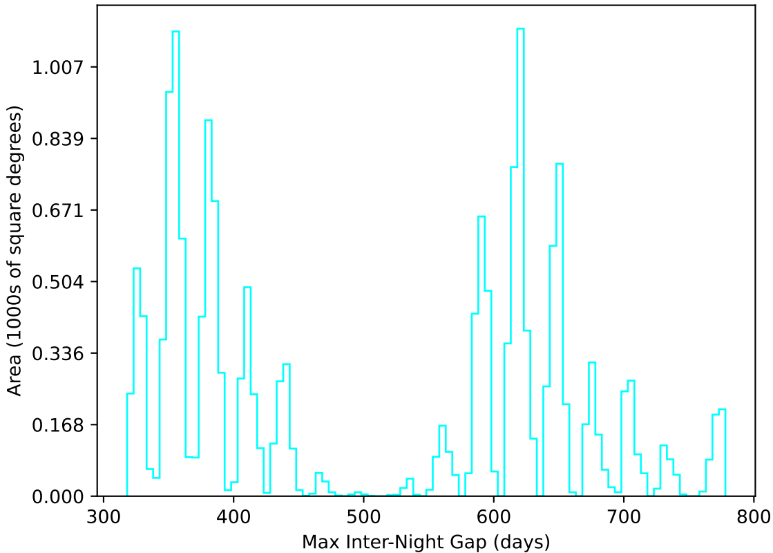
extra_ss_neo3_v3.4_10yrs WFD u band: Max Inter-Night Gap
