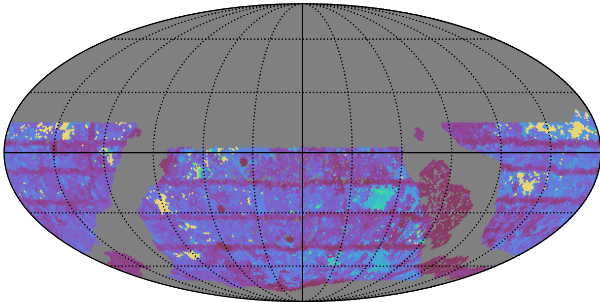
extra_ss_neo3_v3.4_10yrs WFD r band: Max Inter-Night Gap
