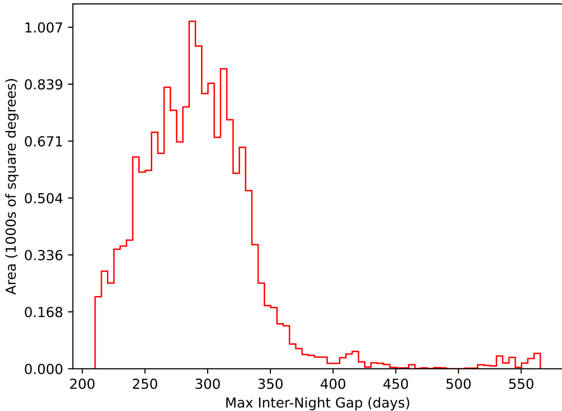
extra_ss_neo3_v3.4_10yrs WFD i band: Max Inter-Night Gap
