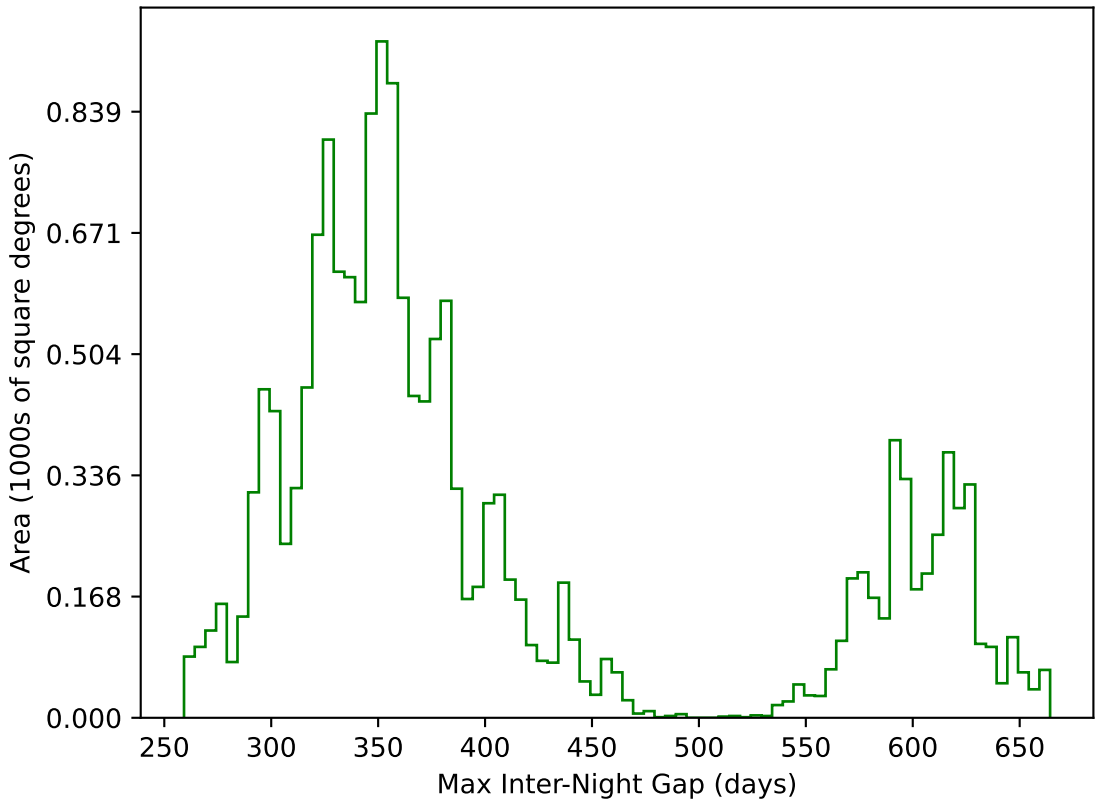
extra_ss_neo3_v3.4_10yrs WFD g band: Max Inter-Night Gap
