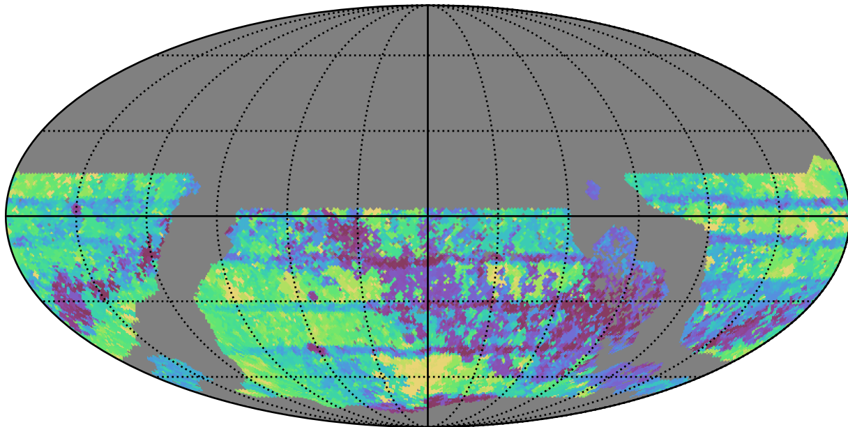
extra_ss_neo3_v3.4_10yrs WFD all bands: Max Inter-Night Gap
