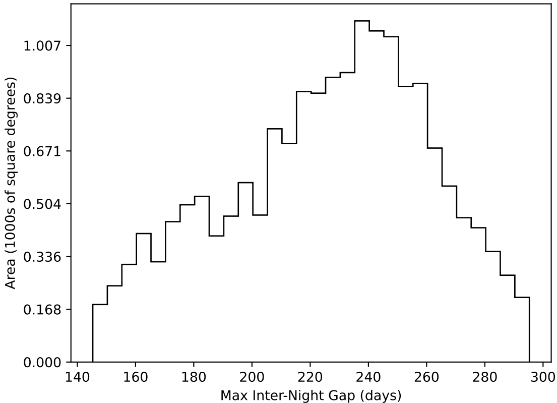
extra_ss_neo3_v3.4_10yrs WFD all bands: Max Inter-Night Gap
