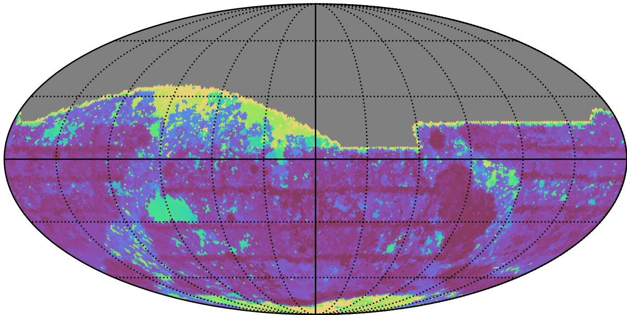
extra_ss_neo3_v3.4_10yrs All sky z band: Max Inter-Night Gap
