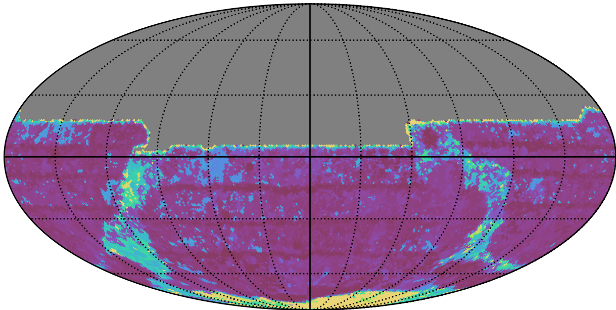
extra_ss_neo3_v3.4_10yrs All sky y band: Max Inter-Night Gap
