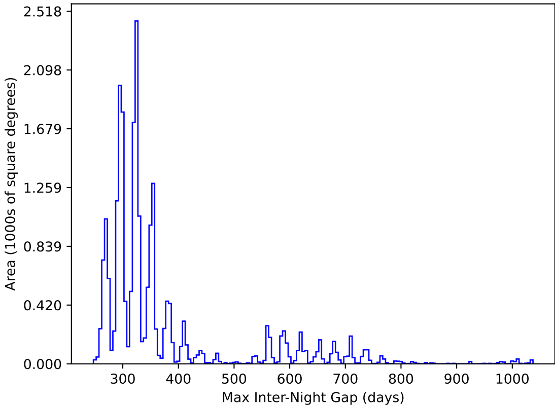
extra_ss_neo3_v3.4_10yrs All sky y band: Max Inter-Night Gap
