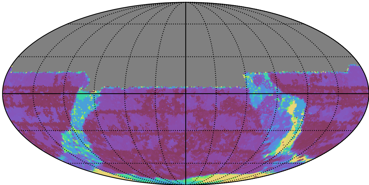
extra_ss_neo3_v3.4_10yrs All sky u band: Max Inter-Night Gap
