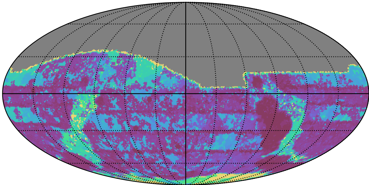
extra_ss_neo3_v3.4_10yrs All sky g band: Max Inter-Night Gap
