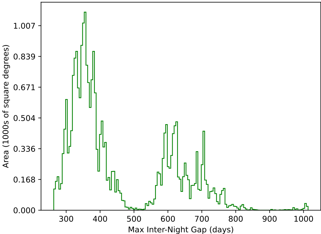
extra_ss_neo3_v3.4_10yrs All sky g band: Max Inter-Night Gap
