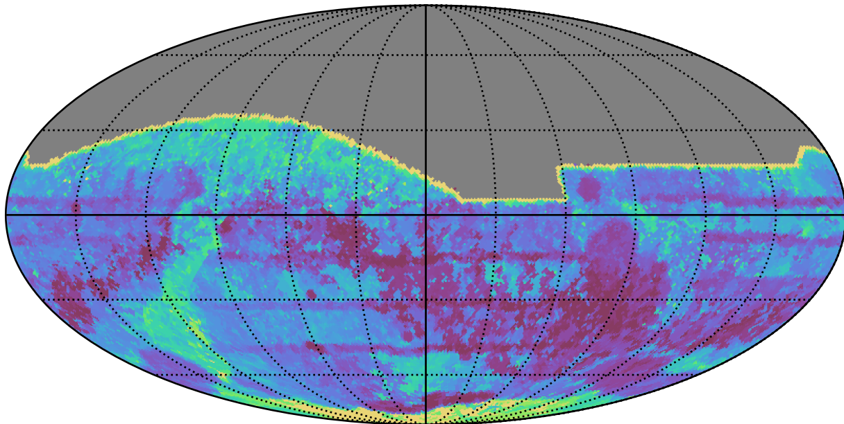
extra_ss_neo3_v3.4_10yrs All sky all bands: Max Inter-Night Gap
