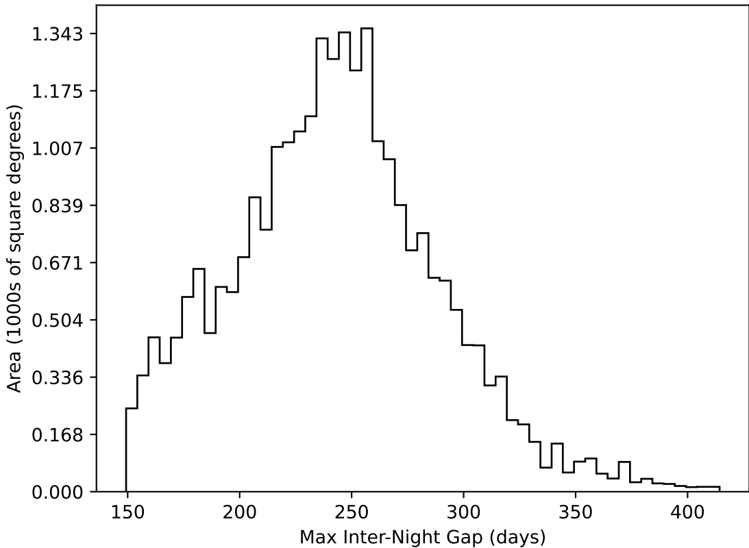
extra_ss_neo3_v3.4_10yrs All sky all bands: Max Inter-Night Gap
