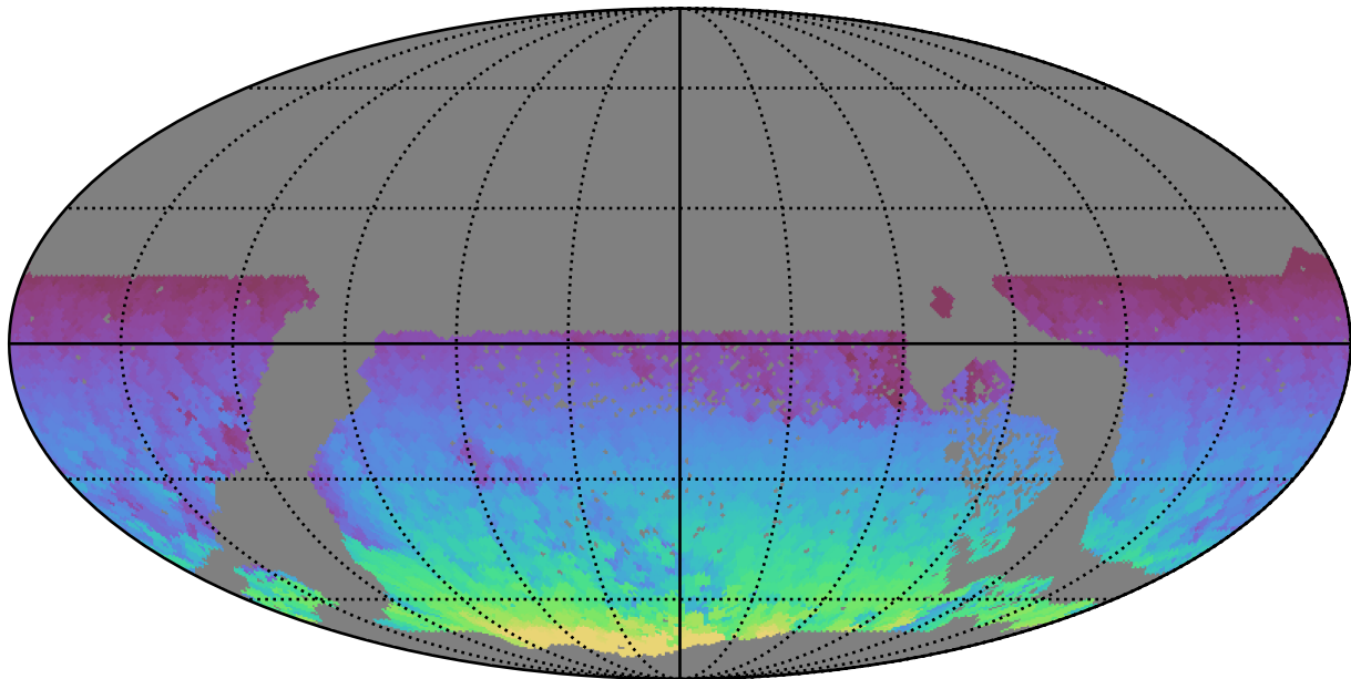
extra_ss_neo3_v3.4_10yrs WFD all bands: Max HA
