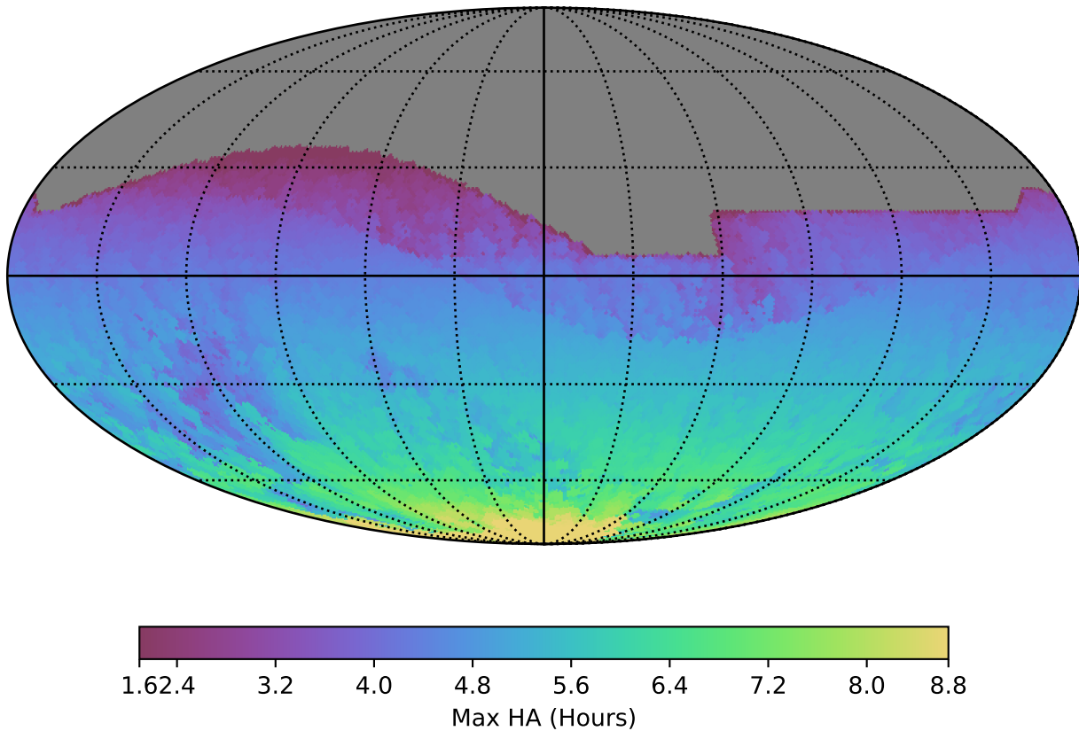
extra_ss_neo3_v3.4_10yrs All sky all bands: Max HA
