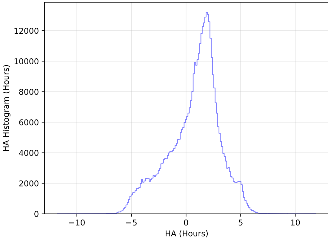
extra_ss_neo3_v3.4_10yrs WFD z band: HA Histogram
