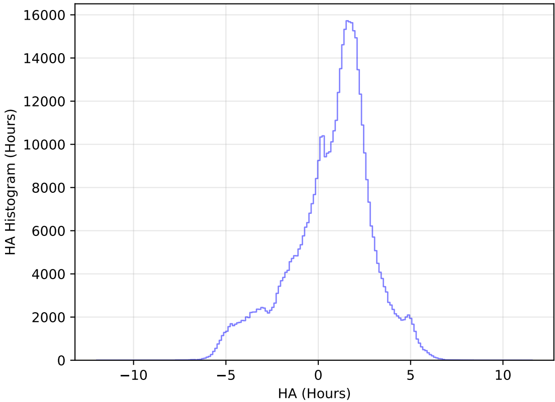
extra_ss_neo3_v3.4_10yrs WFD i band: HA Histogram
