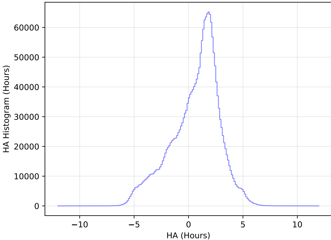
extra_ss_neo3_v3.4_10yrs WFD all bands: HA Histogram
