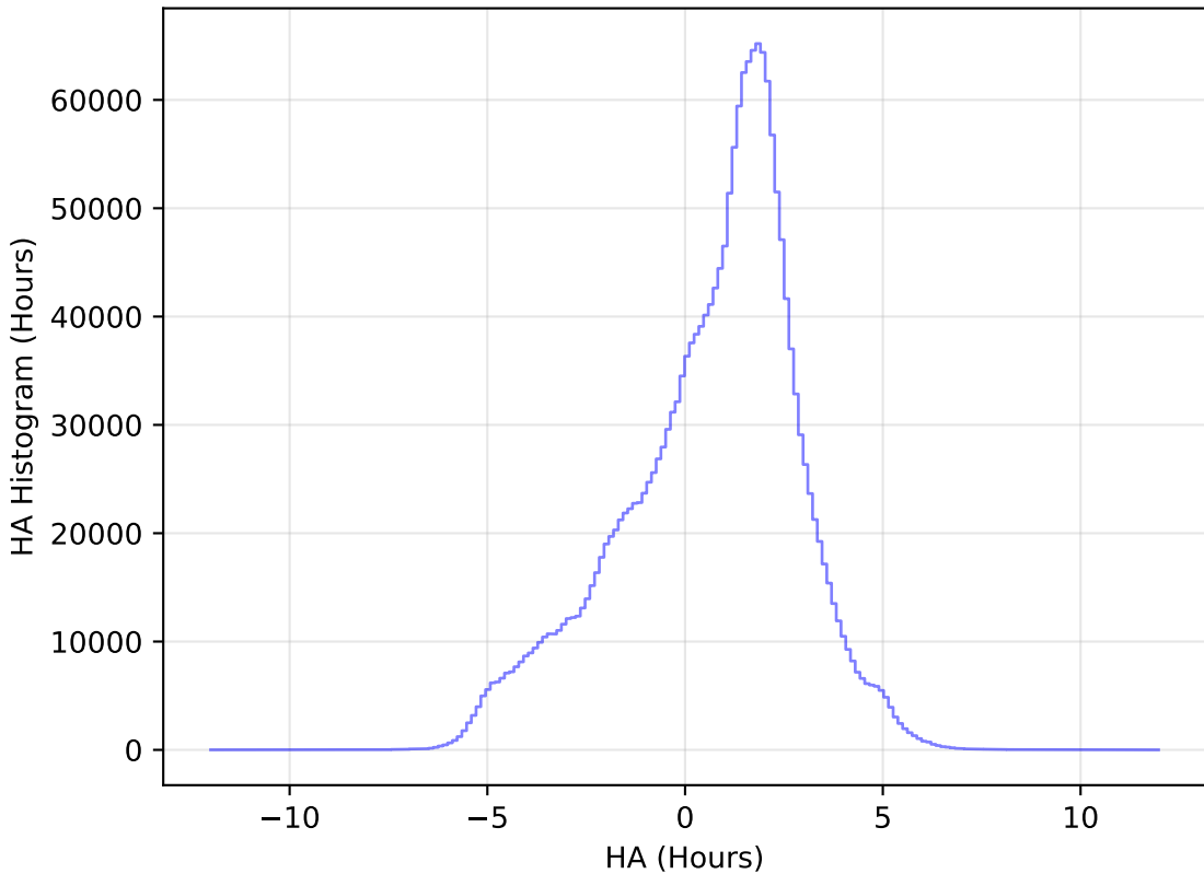
extra_ss_neo3_v3.4_10yrs All sky all bands: HA Histogram
