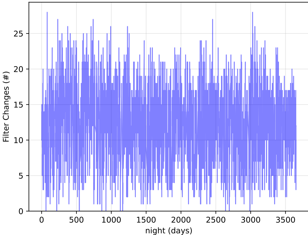
extra_ss_neo3_v3.4_10yrs Per Night: Filter Changes
