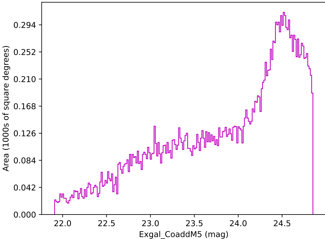
extra_ss_neo3_v3.4_10yrs Yr 3-4 z band: Exgal_CoaddM5
