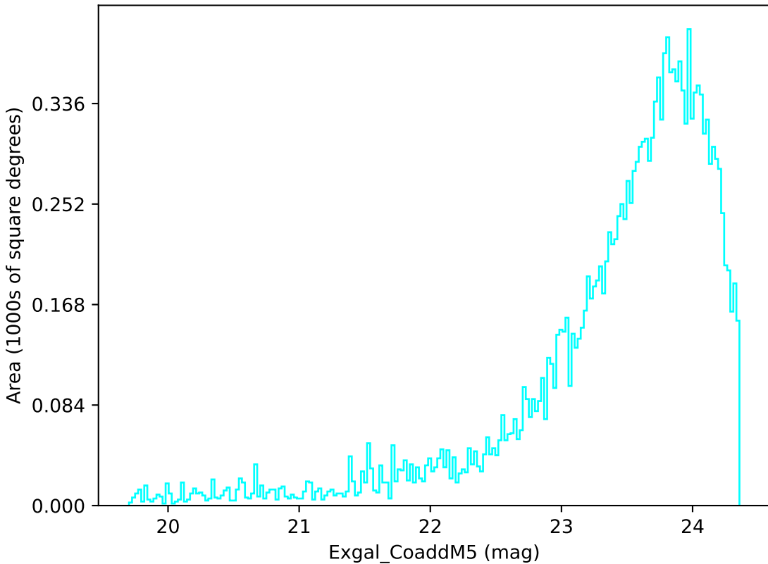
extra_ss_neo3_v3.4_10yrs Yr 3-4 u band: Exgal_CoaddM5
