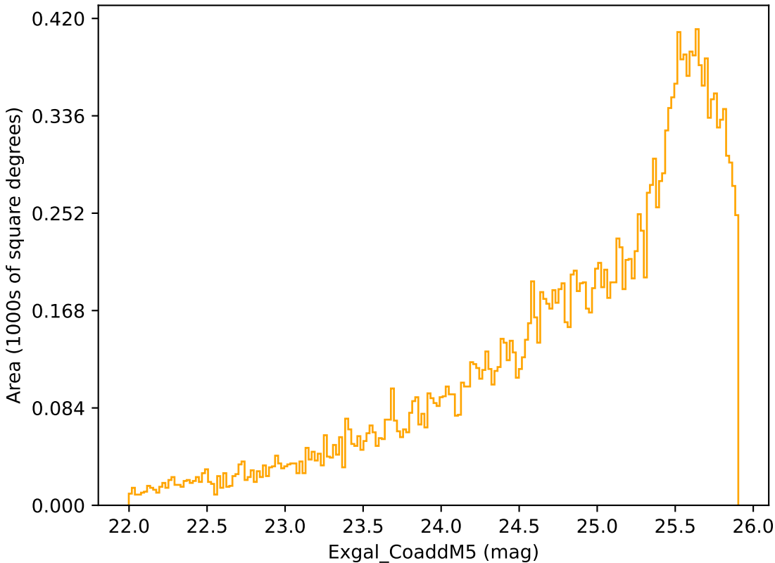
extra_ss_neo3_v3.4_10yrs Yr 3-4 r band: Exgal_CoaddM5
