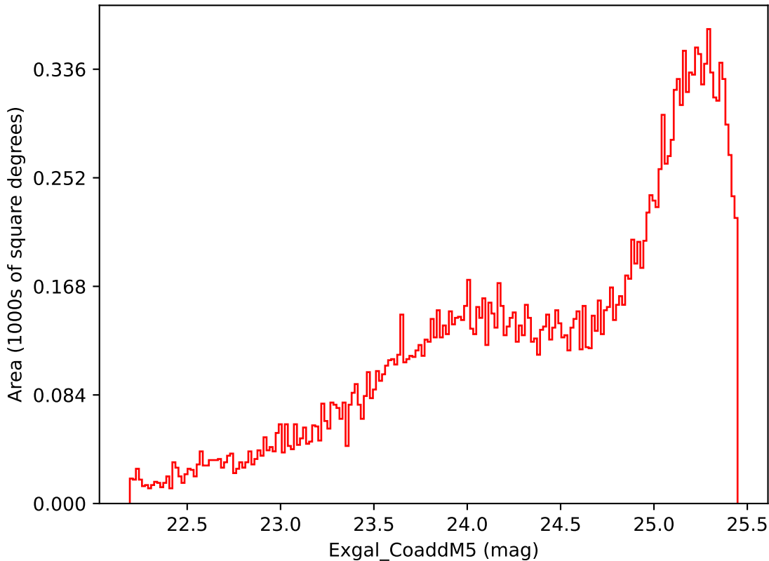
extra_ss_neo3_v3.4_10yrs Yr 3-4 i band: Exgal_CoaddM5
