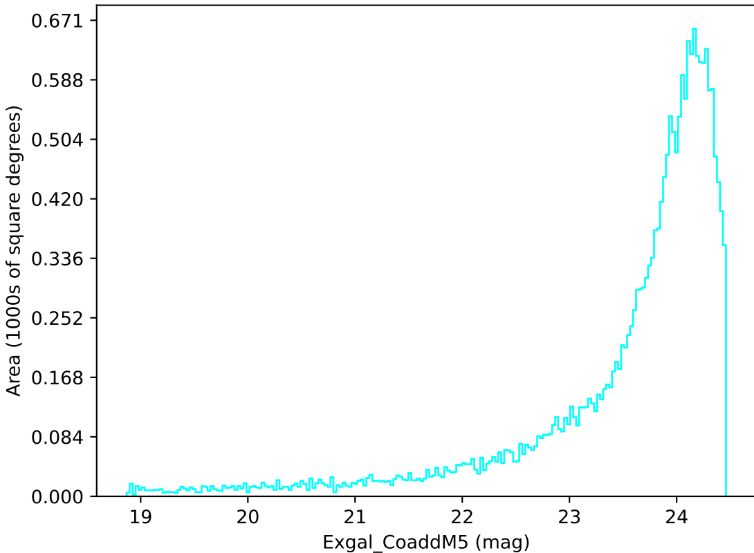
extra_ss_neo3_v3.4_10yrs Yr 1 u band: Exgal_CoaddM5
