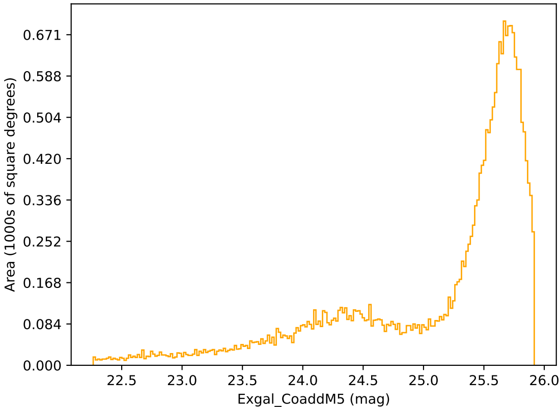
extra_ss_neo3_v3.4_10yrs Yr 1 r band: Exgal_CoaddM5
