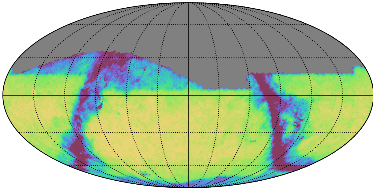
extra_ss_neo3_v3.4_10yrs Yr 1 i band: Exgal_CoaddM5
