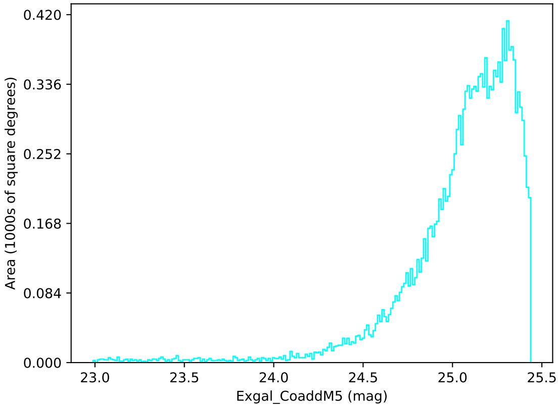
extra_ss_neo3_v3.4_10yrs WFD u band: Exgal_CoaddM5
