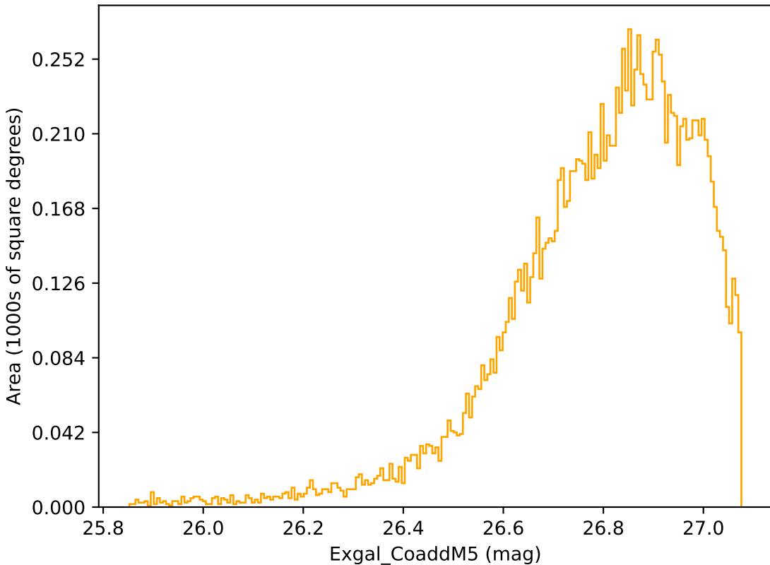
extra_ss_neo3_v3.4_10yrs WFD r band: Exgal_CoaddM5
