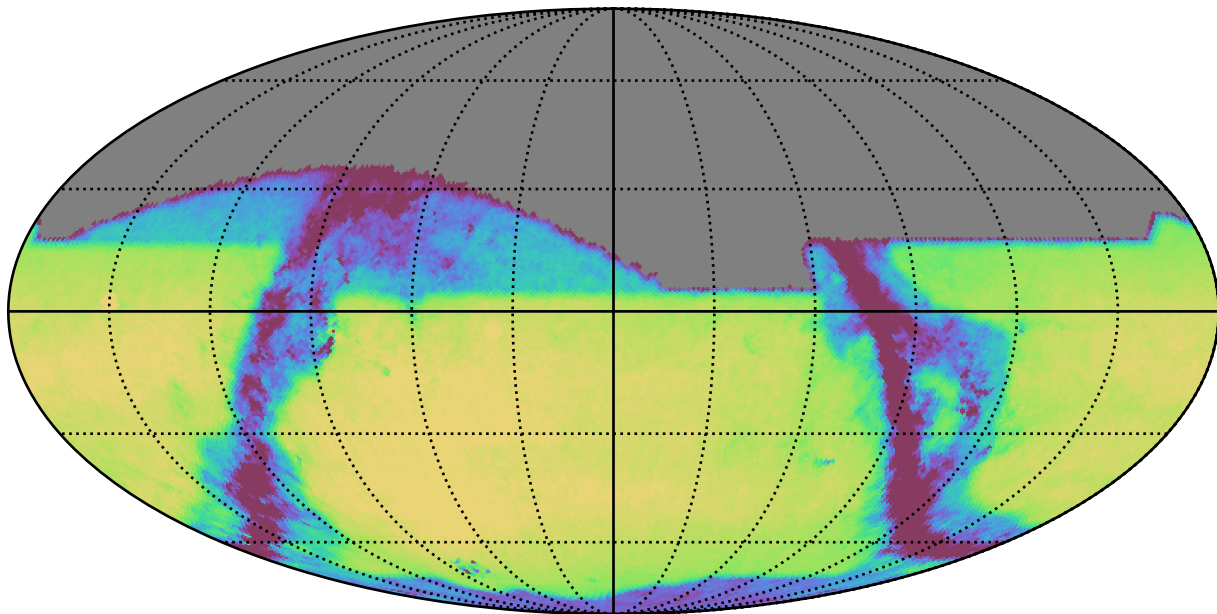
extra_ss_neo3_v3.4_10yrs All sky z band: Exgal_CoaddM5
